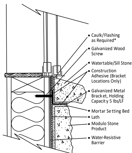
Windowsill Cross Section
